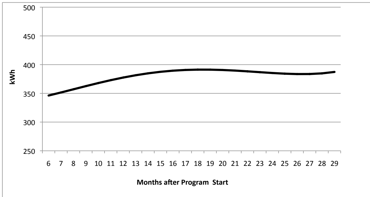
Figure E1. Trend in annual program savings, HC households, program months 6-29 (September 2009-August 2010).
