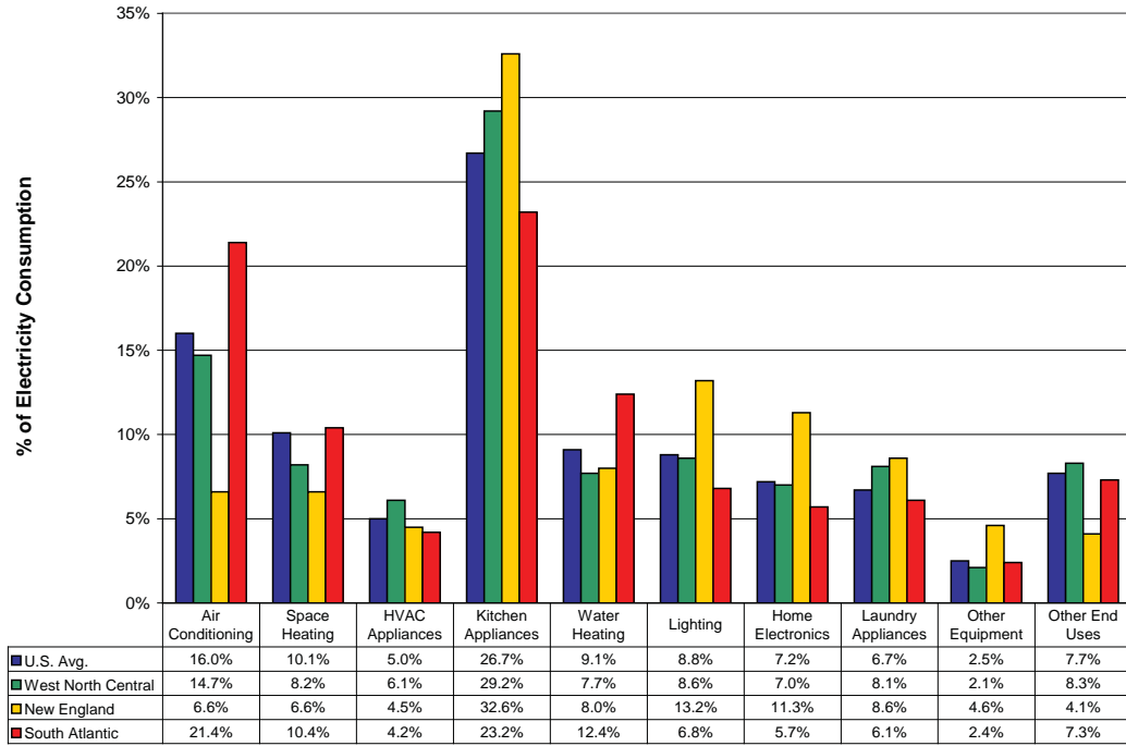
Figure 11: Residential End Use Share of Electricity Consumption by Region (Source: EIA)
