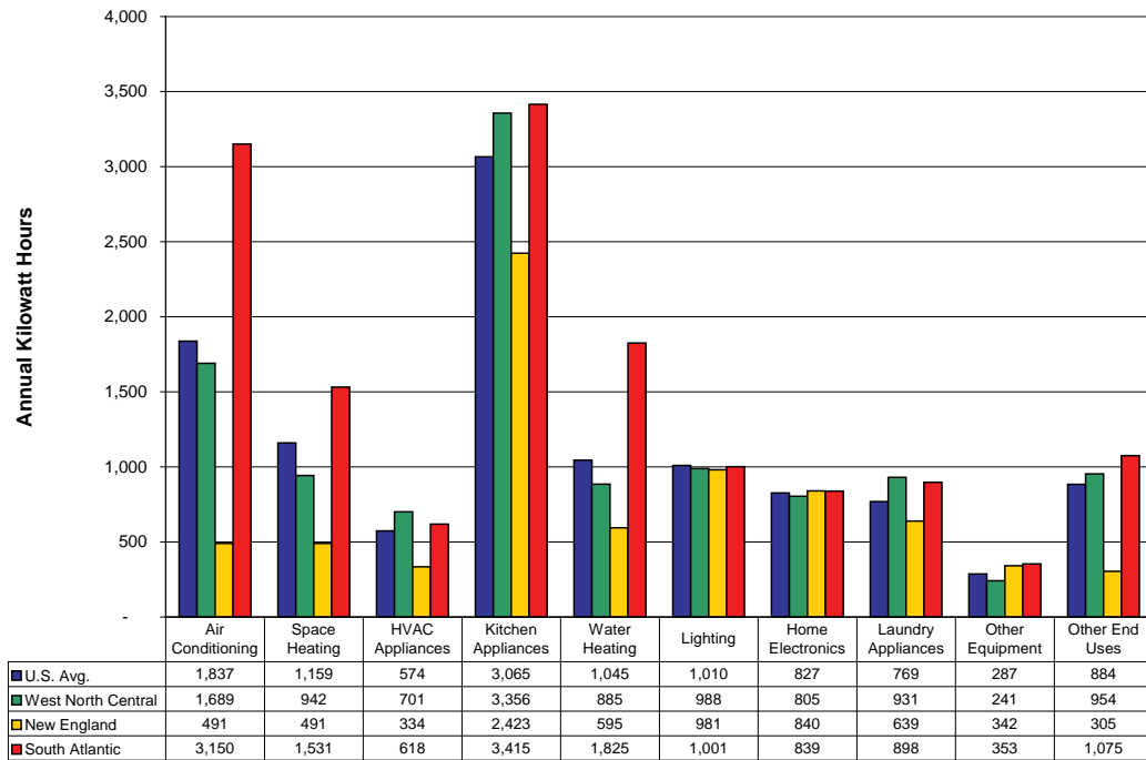
Figure 12: Average Household End Use Electricity Consumption by Region (Source: EIA)
